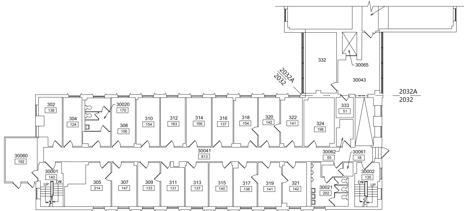
THIRD FLOOR PLAN GROSS AREA = 5,574 SQ. FT.
